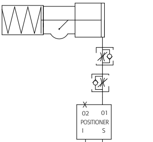
3-15 instrument signal / 4-20 mA instrument signal
