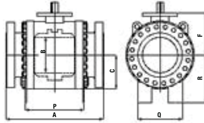
REDUCED BORE
