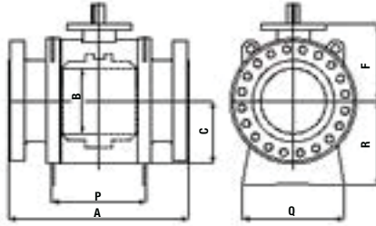
FULL BORE
