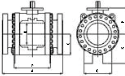
REDUCED BORE
