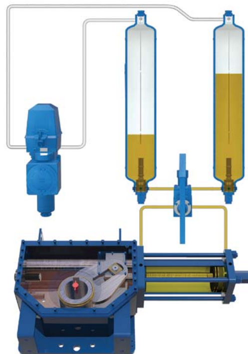
Operational diagram.
