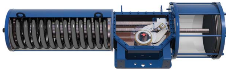
Pneumatic spring return.
