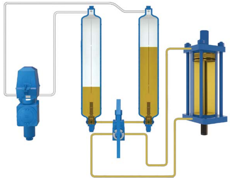
Operational diagram.
