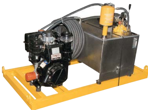
Portable gasoline-operated unit.
