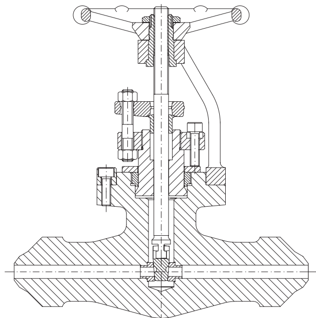
Body Bonnet connection pressure seal design.
