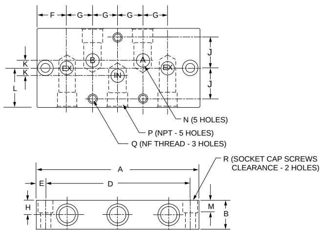
SIDE-PORTED
