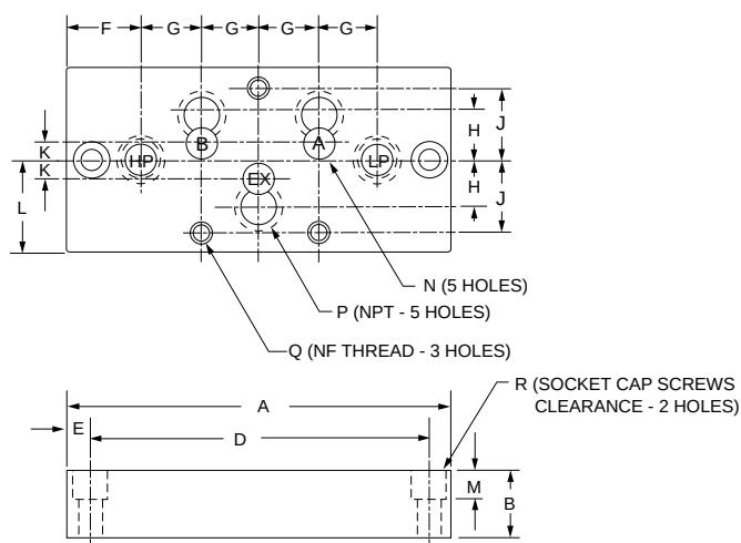
BOTTOM PORTED
