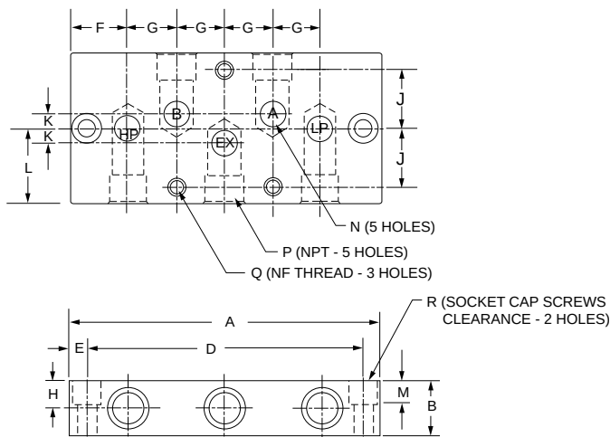
SIDE-PORTED
