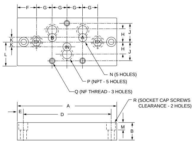
BOTTOM PORTED
