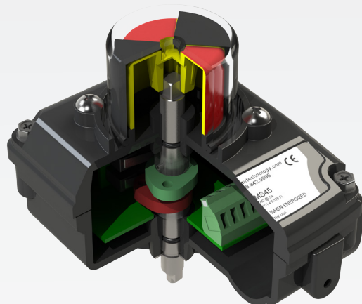
Cutaway View
