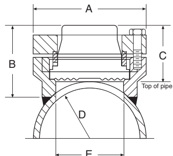
Types 105, 205 – Saddle – 3" Pipe Only Saddle
