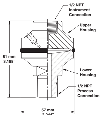
Type 510 – All Welded Threaded Diaphragm Seal
