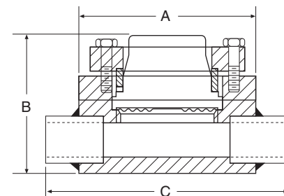
Types 108, 208 – Butt-Welded – (Clamped Design) Process Connection – ¼", ½", ¾", 1", 1½", 2"
