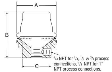
Type 501 – All Welded Threaded Process Connection \frac{1}{4} , \frac{1}{2} , \frac{3}{4} , 1 NPT with flushing connection
