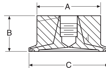
Type 320 Quick Connect – ¼", ½" NPT
