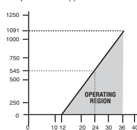
Load Limitations 4-20mA Output Loop Resistance ( )
