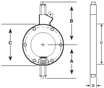
Type 85 Isolation Spool – 1", 1½"
