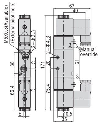
4V220(Terminal)
