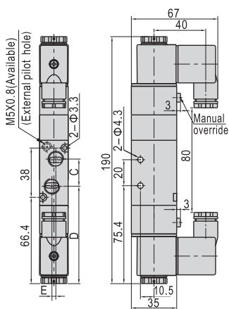
4V230(Terminal)
