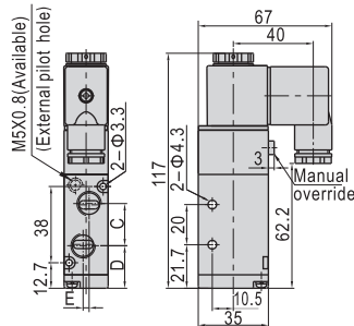
4V210(Terminal)
